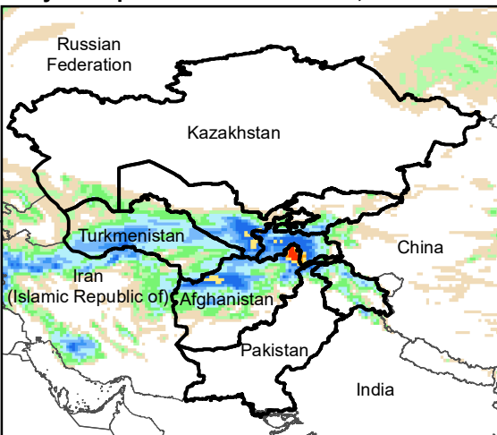
Daily Precip. Forecast for 20 Feb., 2024
