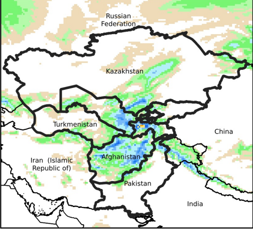
Daily Precip. Forecast for Mar 11, 2024
