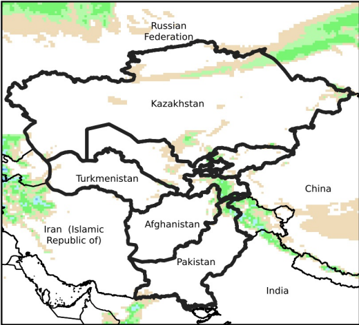
Daily Precip. Forecast for Mar 10, 2024
