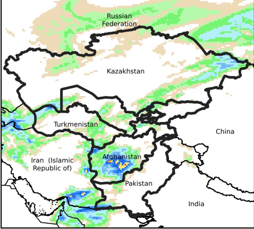
Daily Precip. Forecast for Mar 10, 2024
