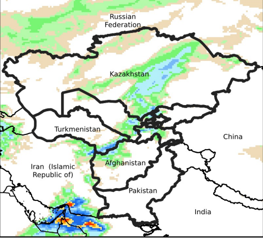
Daily Precip. Forecast for Mar 9, 2024
