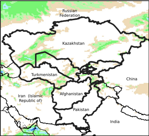
Daily Precip. Forecast for Mar 11, 2024
