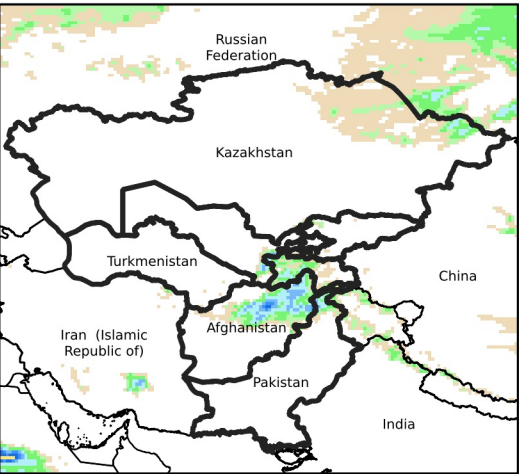
Daily Precip. Forecast for Apr 5, 2024
