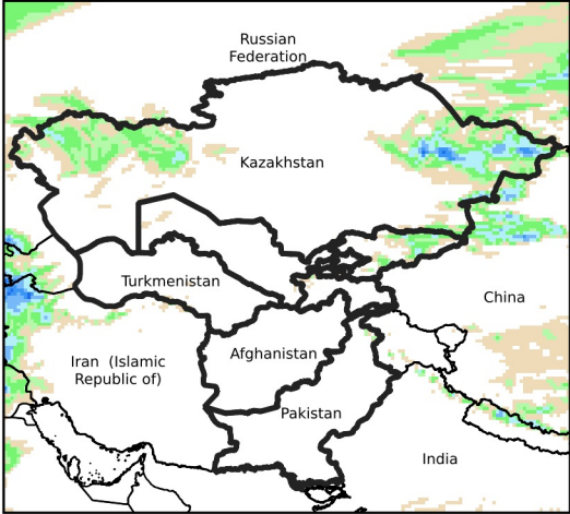
Daily Precip. Forecast for Apr 7, 2024
