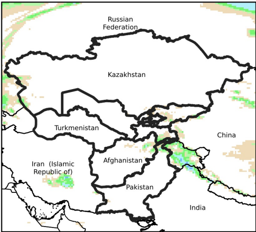
Daily Precip. Forecast for Apr 7, 2024
