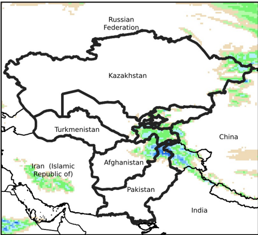
Daily Precip. Forecast for Apr 6, 2024
