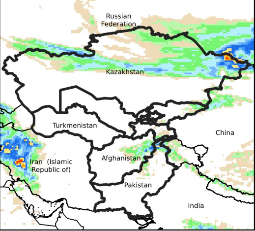
Daily Precip. Forecast for Apr 10, 2024
