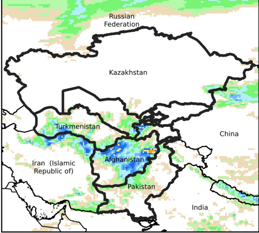
Daily Precip. Forecast for Apr 12, 2024
