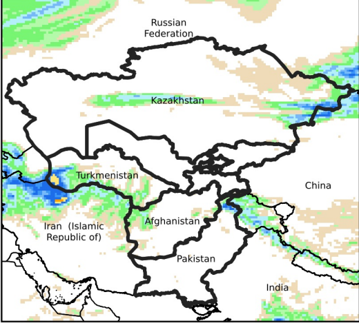
Daily Precip. Forecast for Apr 11, 2024
