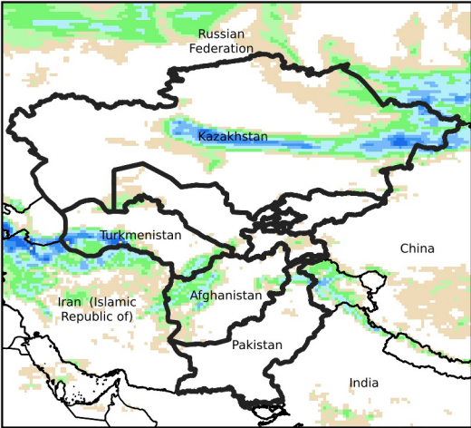
Daily Precip. Forecast for Apr 14, 2024
