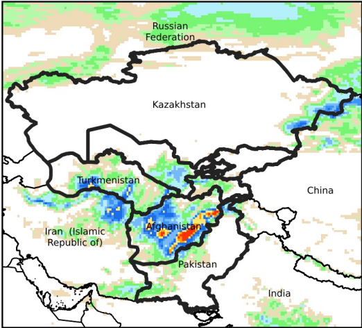
Daily Precip. Forecast for Apr 15, 2024
