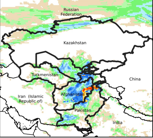
Daily Precip. Forecast for Apr 13, 2024
