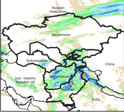
Daily Precip. Forecast for Apr 14, 2024
