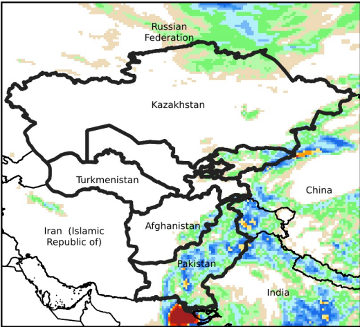
Daily Precip. Forecast for Sep 1, 2024
