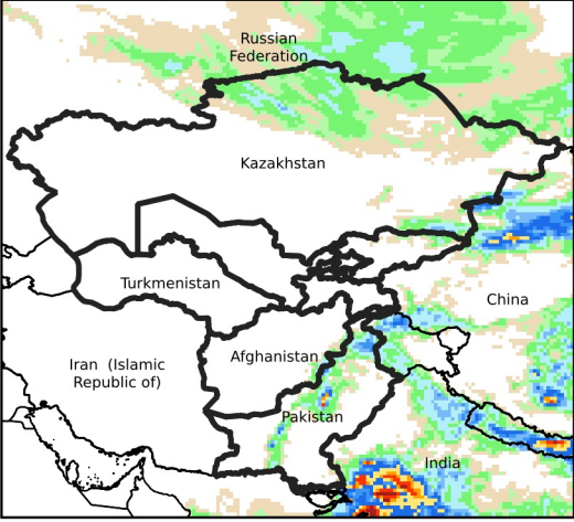
Daily Precip. Forecast for Sep 2, 2024
