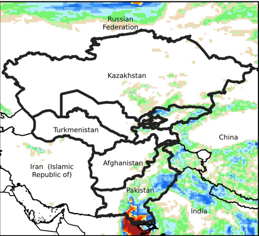
Daily Precip. Forecast for Aug 31, 2024
