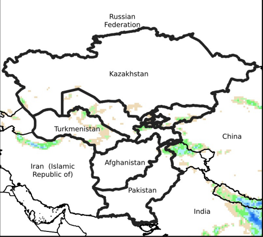
Daily Precip. Forecast for Oct 4, 2024
