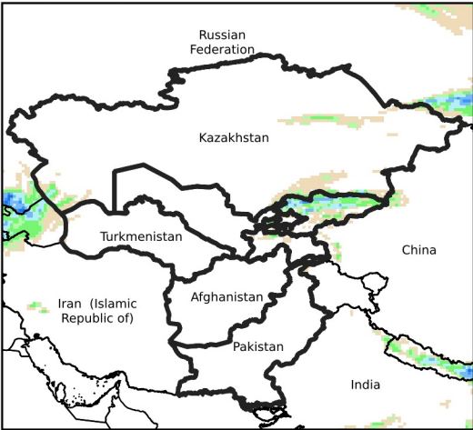
Daily Precip. Forecast for Oct 5, 2024
