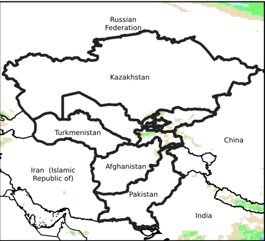
Daily Precip. Forecast for Oct 4, 2024
