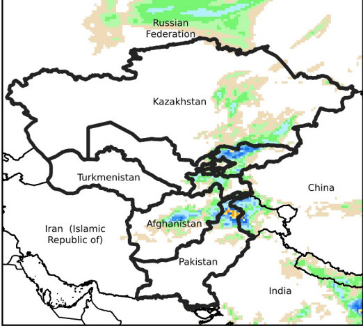
Daily Precip. Forecast for Oct 6, 2024
