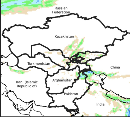
Daily Precip. Forecast for Oct 5, 2024
