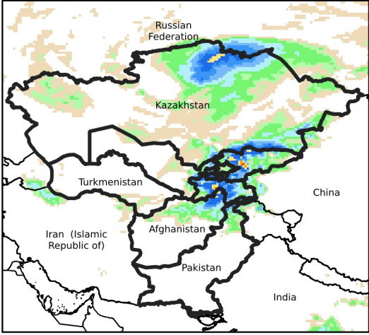
Daily Precip. Forecast for Oct 28, 2024
