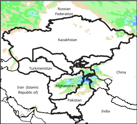
Daily Precip. Forecast for Nov 18, 2024
