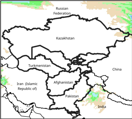
Daily Precip. Forecast for Jan 14, 2025
