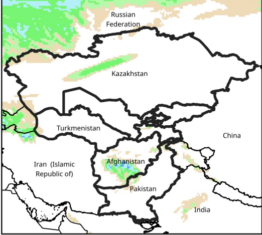
Daily Precip. Forecast for Jan 15, 2025
