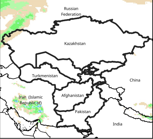
Daily Precip. Forecast for Jan 13, 2025
