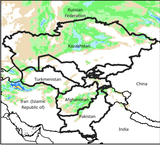
Daily Precip. Forecast for Jan 20, 2025
