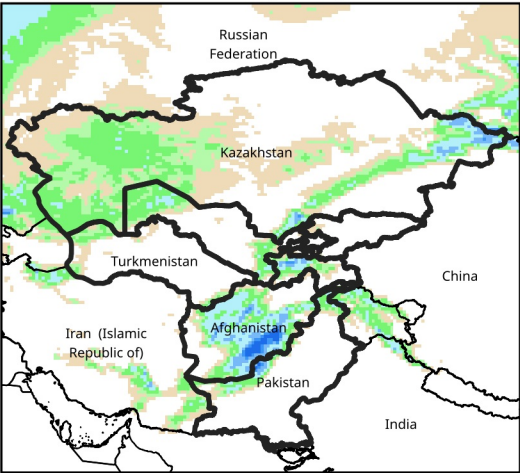
Daily Precip. Forecast for Jan 21, 2025
