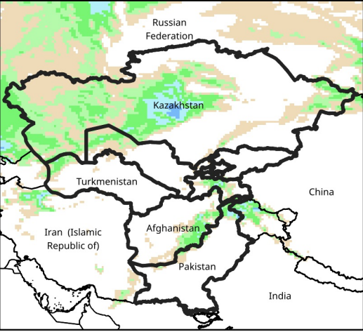
Daily Precip. Forecast for Jan 19, 2025
