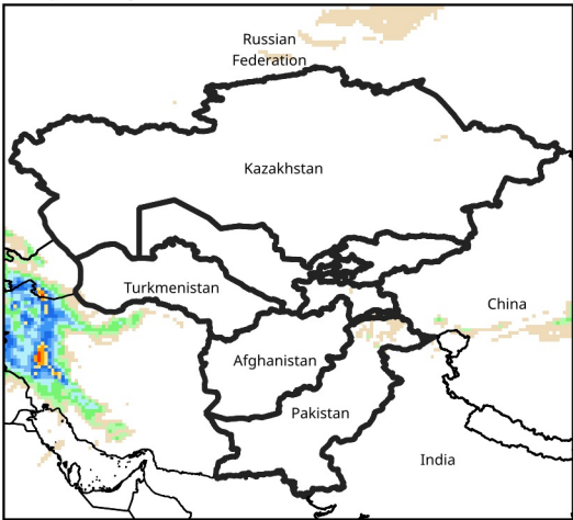
Daily Precip. Forecast for Feb 9, 2025
