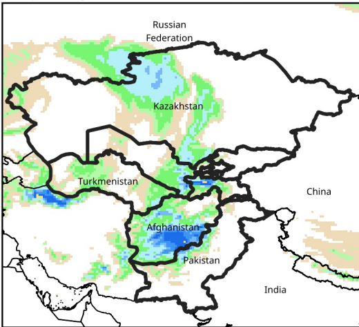
Daily Precip. Forecast for Feb 27, 2025
