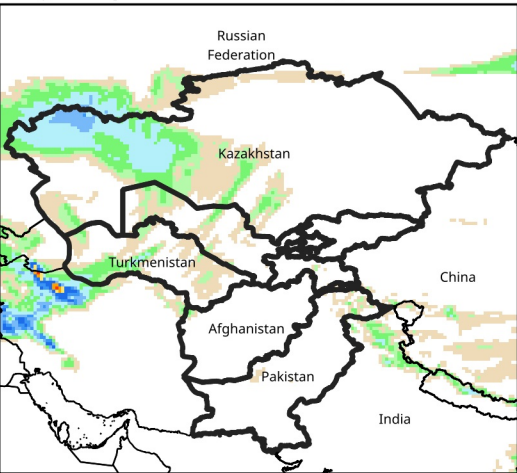
Daily Precip. Forecast for Feb 25, 2025
