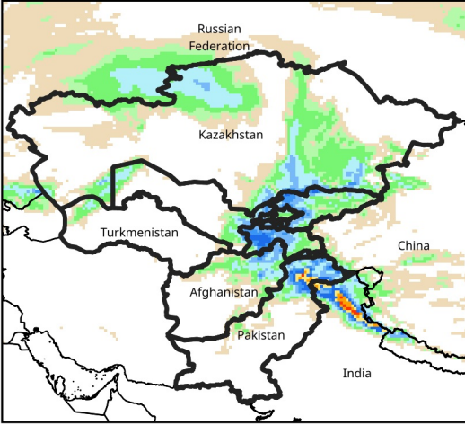
Daily Precip. Forecast for Feb 26, 2025
