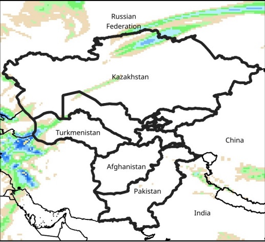
Daily Precip. Forecast for Mar 20, 2025
