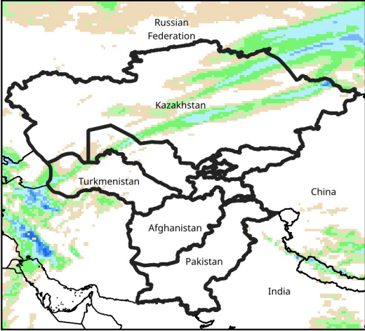
Daily Precip. Forecast for Mar 21, 2025
