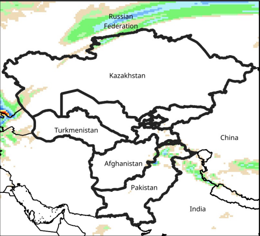
Daily Precip. Forecast for Mar 22, 2025
