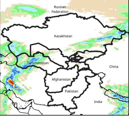
Daily Precip. Forecast for Mar 22, 2025
