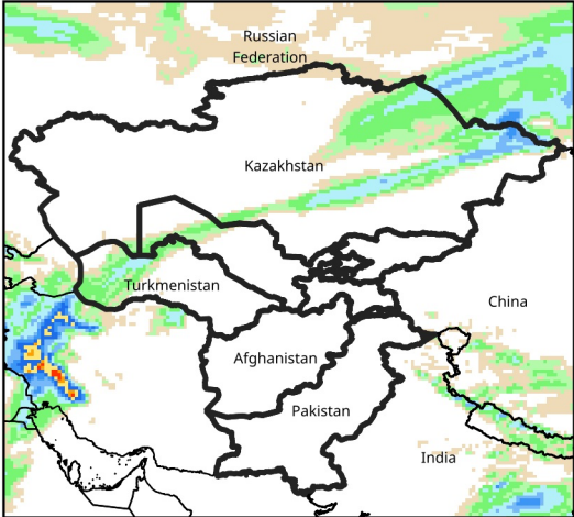
Daily Precip. Forecast for Mar 24, 2025
