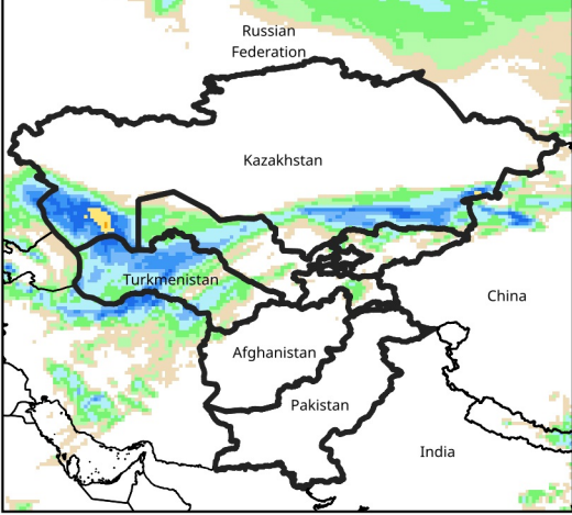
Daily Precip. Forecast for Mar 23, 2025
