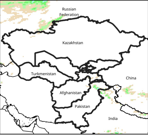
Daily Precip. Forecast for Oct 24, 2025
