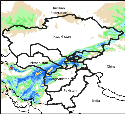
Daily Precip. Forecast for Dec 20, 2025
