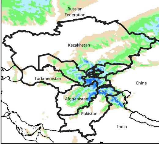
Daily Precip. Forecast for Dec 21, 2025
