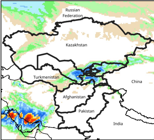
Daily Precip. Forecast for Dec 21, 2025
