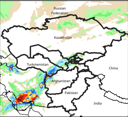
Daily Precip. Forecast for Dec 19, 2025
