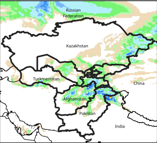
Daily Precip. Forecast for Dec 24, 2025
