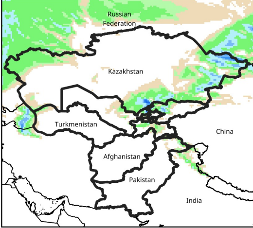
Daily Precip. Forecast for Dec 26, 2025
