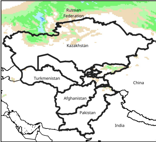
Daily Precip. Forecast for Dec 26, 2025
