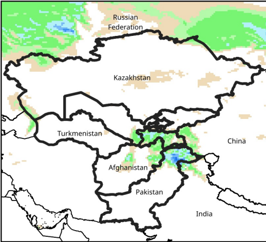
Daily Precip. Forecast for Dec 25, 2025
