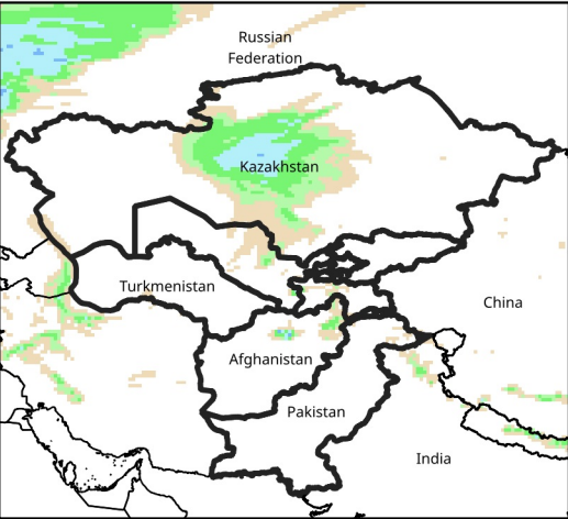
Daily Precip. Forecast for Jan 6, 2026
