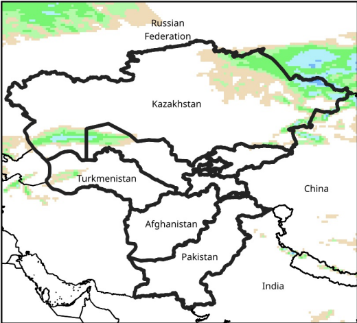
Daily Precip. Forecast for Feb 26, 2026
