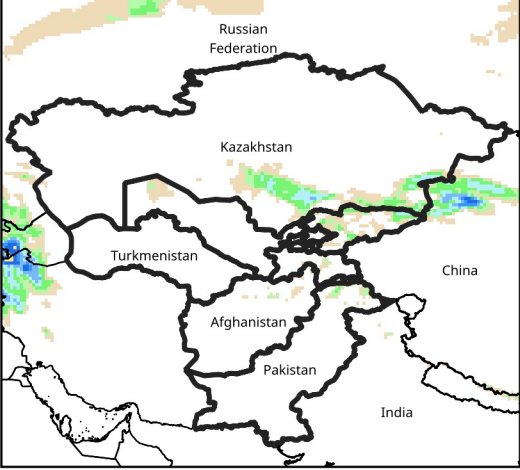
Daily Precip. Forecast for Feb 27, 2026
