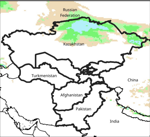
Daily Precip. Forecast for Feb 25, 2026
