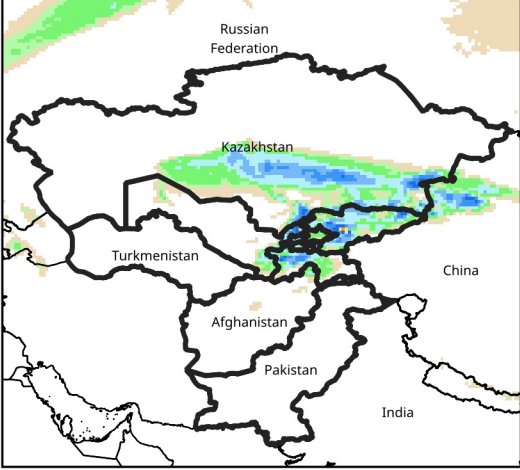
Daily Precip. Forecast for Feb 26, 2026
