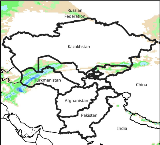
Daily Precip. Forecast for Feb 27, 2026
