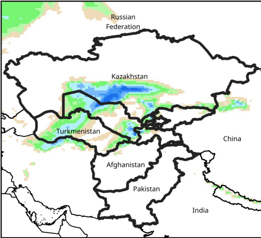
Daily Precip. Forecast for Feb 28, 2026
