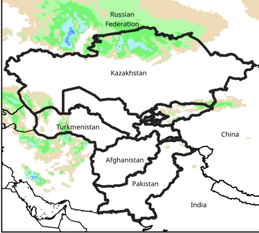
Daily Precip. Forecast for Mar 1, 2026
