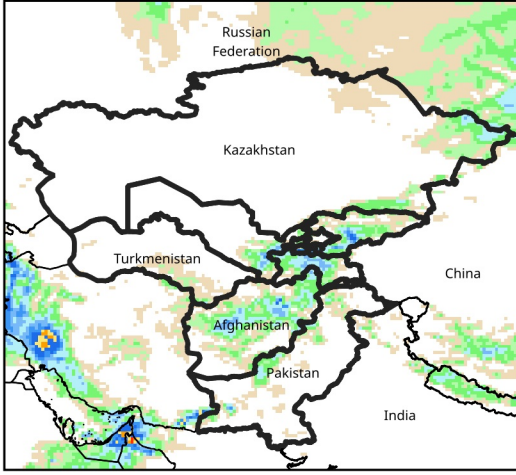
Daily Precip. Forecast for Mar 22, 2026
