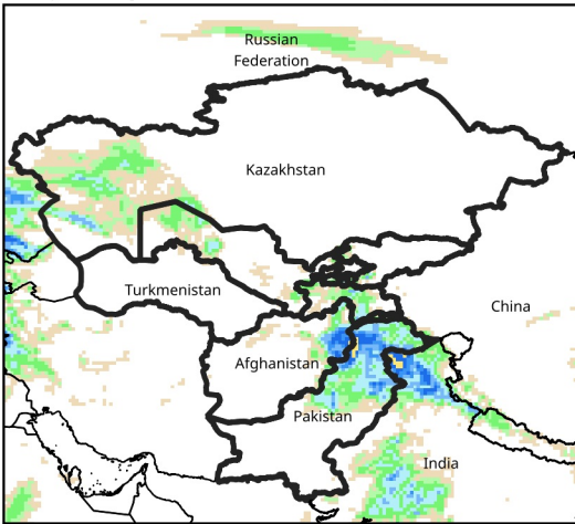
Daily Precip. Forecast for Apr 2, 2026
