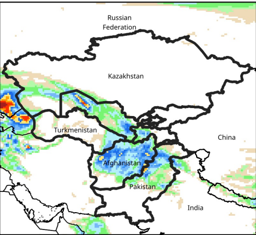
Daily Precip. Forecast for Mar 31, 2026
