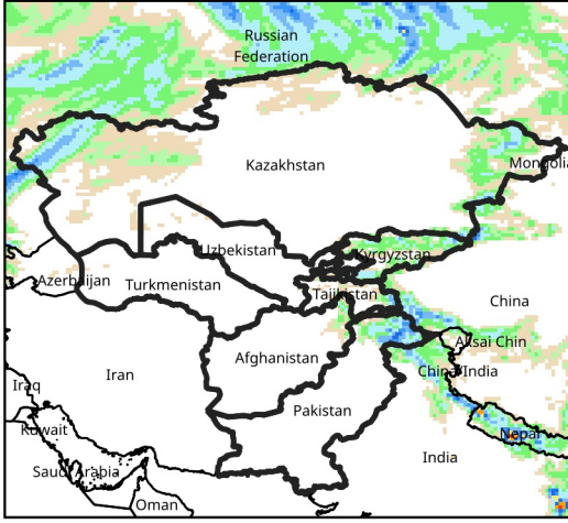
Daily Precip. Forecast for May 28, 2026
