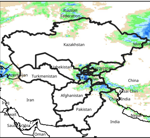
Daily Precip. Forecast for May 27, 2026
