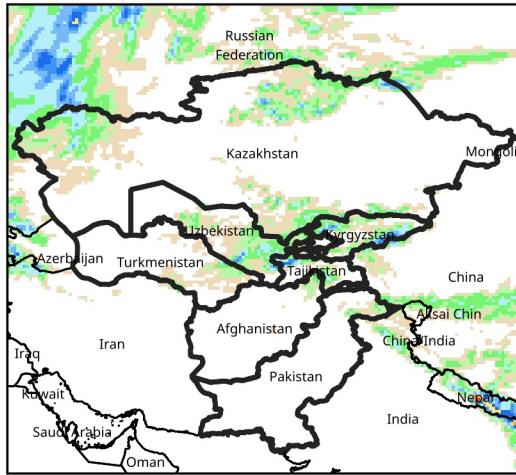
Daily Precip. Forecast for May 29, 2026
