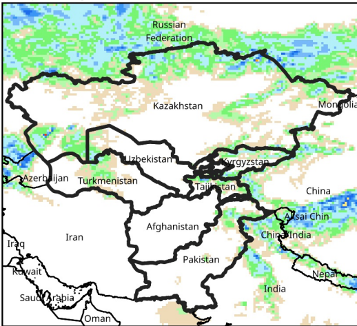
Daily Precip. Forecast for Jun 18, 2026
