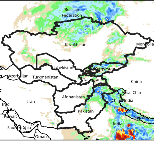
Daily Precip. Forecast for Jul 2, 2026
