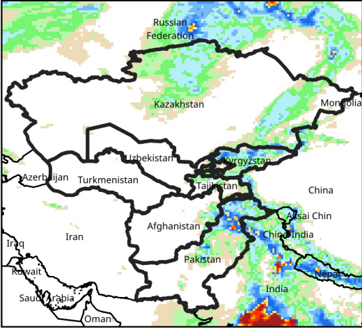
Daily Precip. Forecast for Jul 3, 2026
