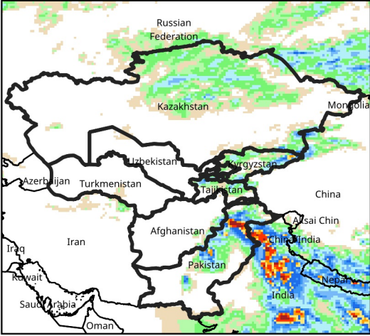
Daily Precip. Forecast for Jul 21, 2026
