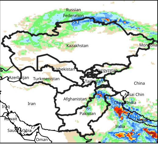
Daily Precip. Forecast for Jul 20, 2026
