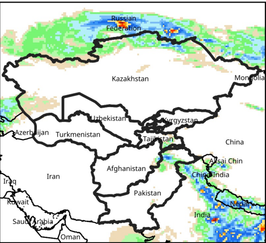
Daily Precip. Forecast for Jul 22, 2026
