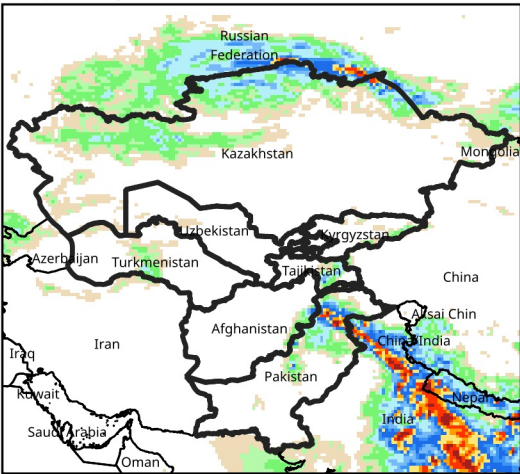
Daily Precip. Forecast for Jul 23, 2026
