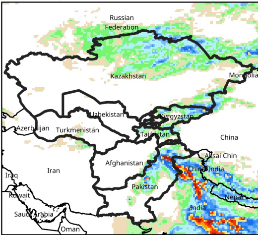
Daily Precip. Forecast for Jul 24, 2026
