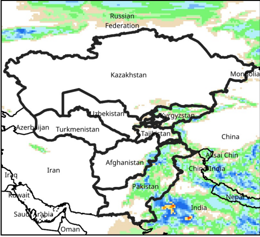
Daily Precip. Forecast for Aug 8, 2026
