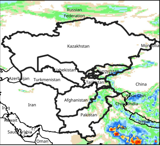
Daily Precip. Forecast for Aug 7, 2026
