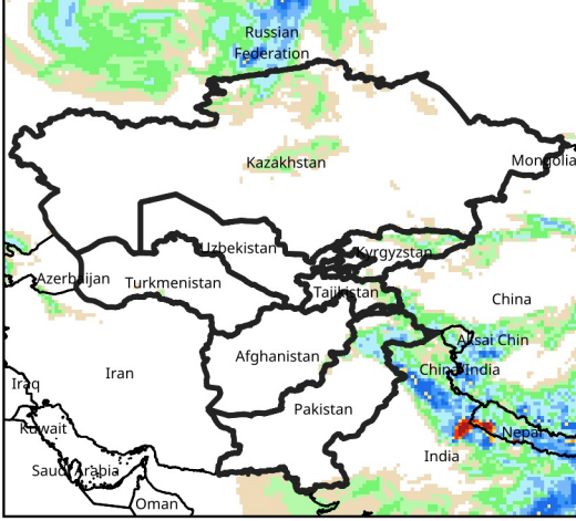
Daily Precip. Forecast for Aug 15, 2026
