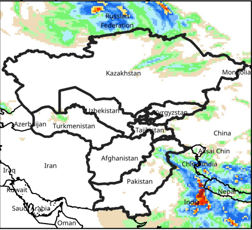
Daily Precip. Forecast for Aug 16, 2026
