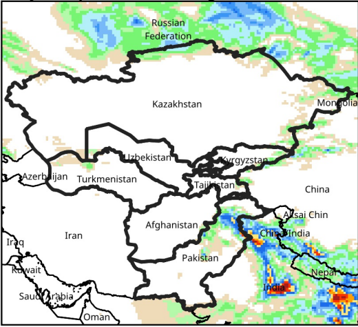
Daily Precip. Forecast for Aug 17, 2026
