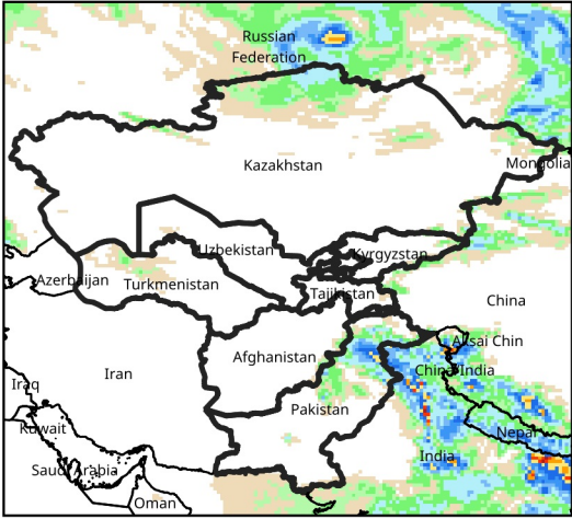
Daily Precip. Forecast for Aug 18, 2026
