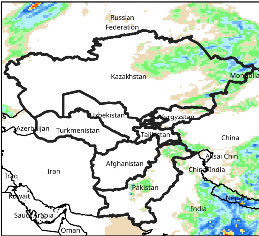
Daily Precip. Forecast for Aug 27, 2026
