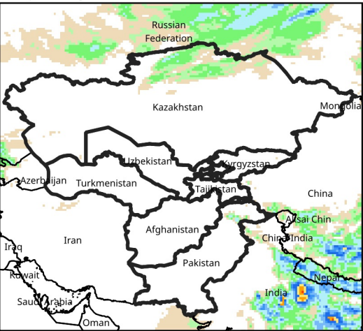
Daily Precip. Forecast for Aug 30, 2026
