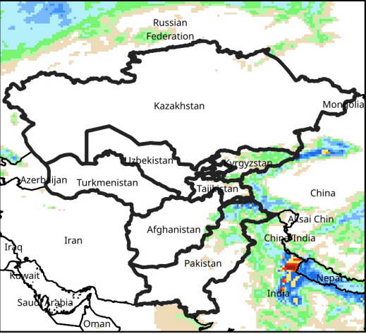
Daily Precip. Forecast for Sep 5, 2026
