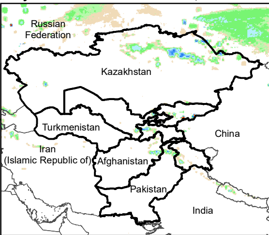
Daily Rainfall estimate for 26 Nov., 2002
