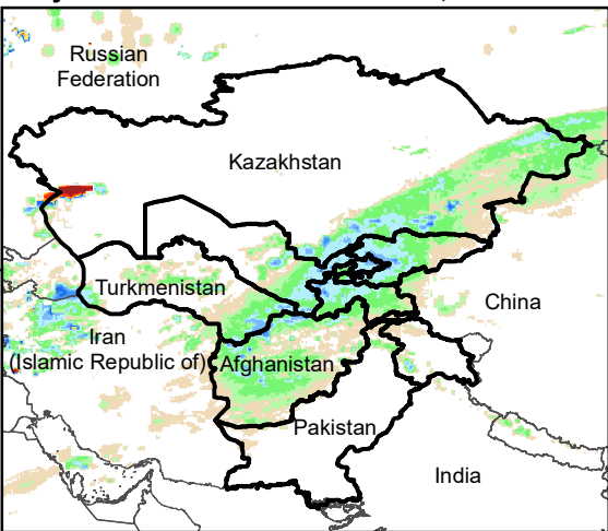
Daily Rainfall estimate for 15 Dec., 2002
