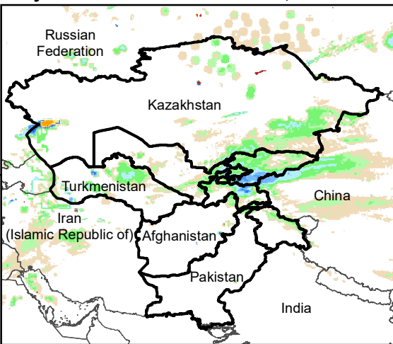
Daily Rainfall estimate for 20 Dec., 2002
