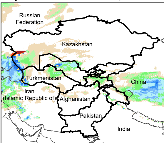
Daily Rainfall estimate for 21 Dec., 2002
