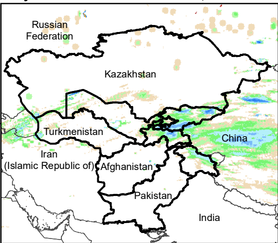
Daily Rainfall estimate for 19 Dec., 2002
