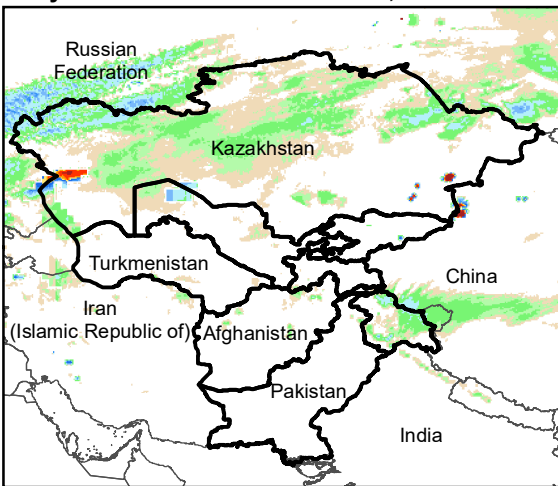
Daily Rainfall estimate for 12 Jan., 2003
