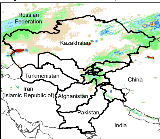
Daily Rainfall estimate for 11 Jan., 2003
