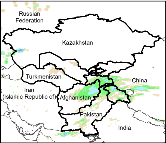
Daily Rainfall estimate for 26 Jan., 2003
