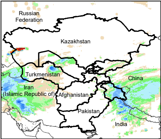
Daily Rainfall estimate for 28 Jan., 2003
