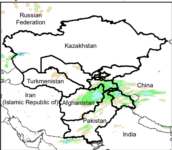
Daily Rainfall estimate for 29 Jan., 2003
