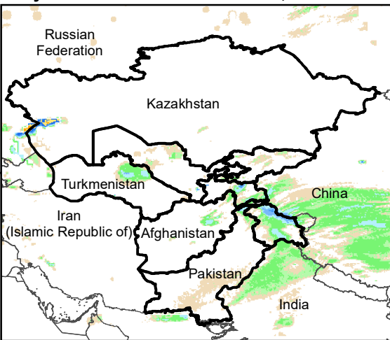
Daily Rainfall estimate for 30 Jan., 2003
