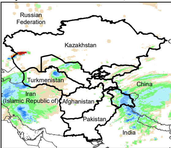
Daily Rainfall estimate for 31 Jan., 2003
