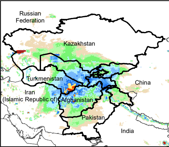
Daily Rainfall estimate for 17 Mar., 2003
