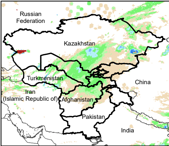
Daily Rainfall estimate for 18 Mar., 2003
