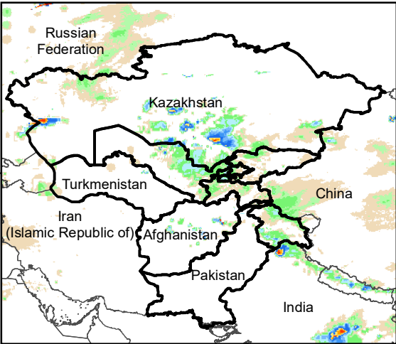
Daily Rainfall estimate for 16 Mar., 2003
