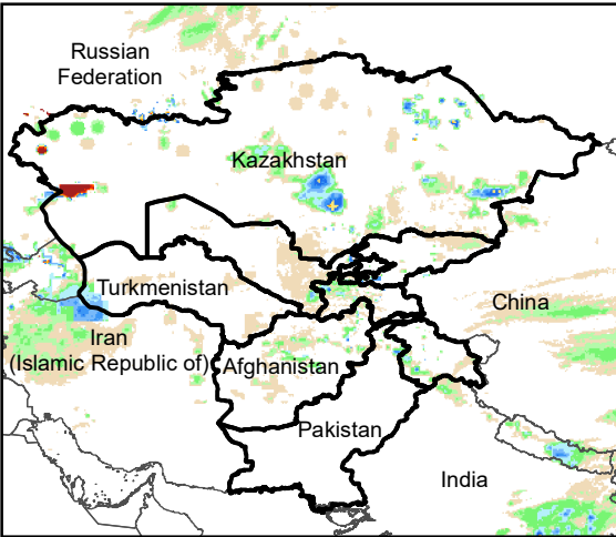
Daily Rainfall estimate for 17 Mar., 2003
