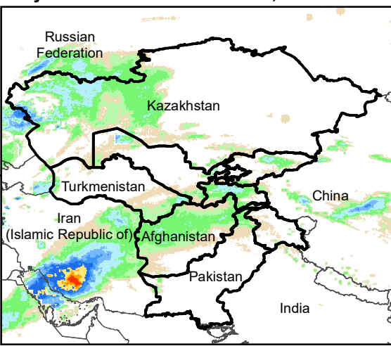
Daily Rainfall estimate for 9 Jan., 2004
