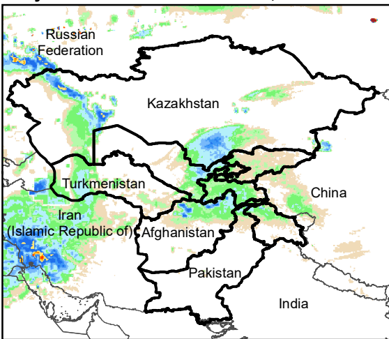
Daily Rainfall estimate for 10 Jan., 2004
