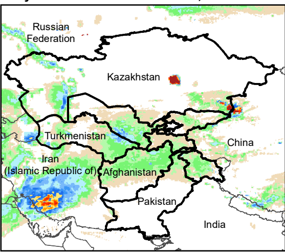
Daily Rainfall estimate for 8 Jan., 2004
