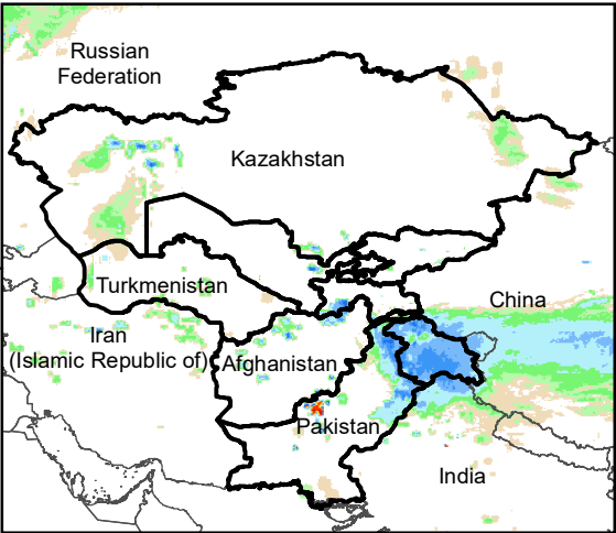
Daily Rainfall estimate for 30 Jan., 2004
