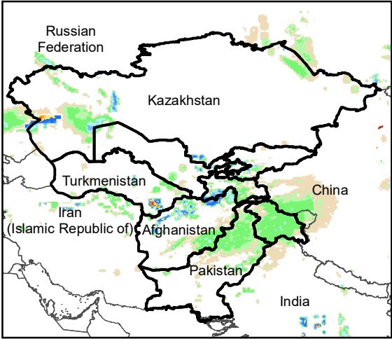
Daily Rainfall estimate for 1 Feb., 2004
