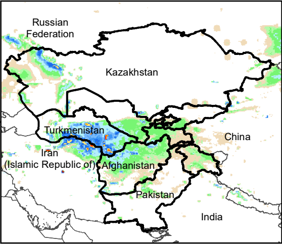
Daily Rainfall estimate for 31 Jan., 2004
