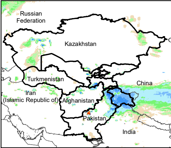
Daily Rainfall estimate for 2 Feb., 2004
