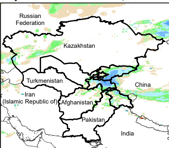
Daily Rainfall estimate for 21 Feb., 2004
