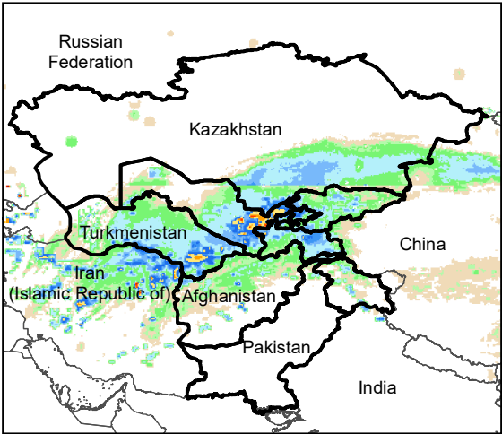
Daily Rainfall estimate for 15 Mar., 2004
