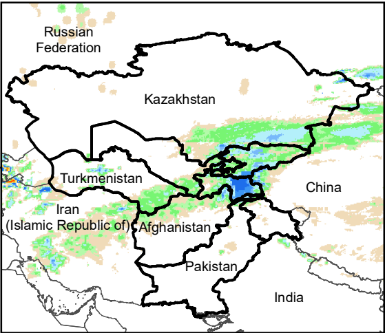
Daily Rainfall estimate for 13 Mar., 2004
