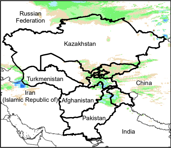
Daily Rainfall estimate for 14 Mar., 2004
