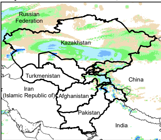
Daily Rainfall estimate for 1 Apr., 2004
