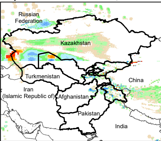
Daily Rainfall estimate for 31 Mar., 2004
