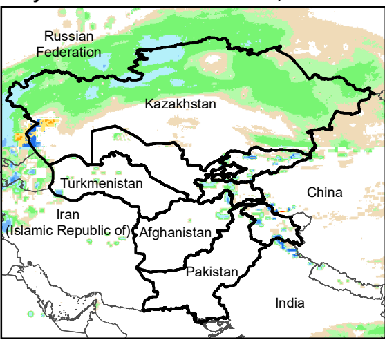
Daily Rainfall estimate for 30 Mar., 2004
