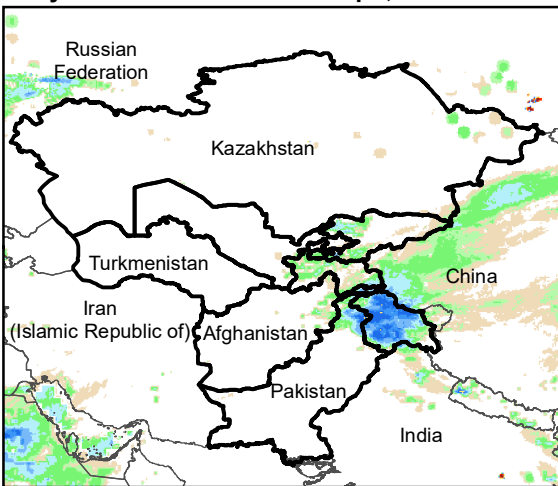
Daily Rainfall estimate for 12 Apr., 2004
