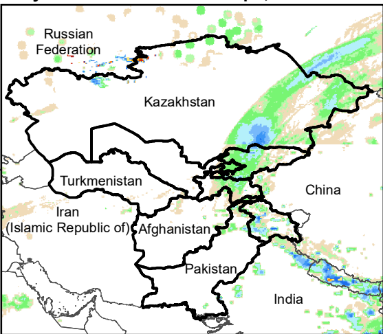
Daily Rainfall estimate for 10 Apr., 2004
