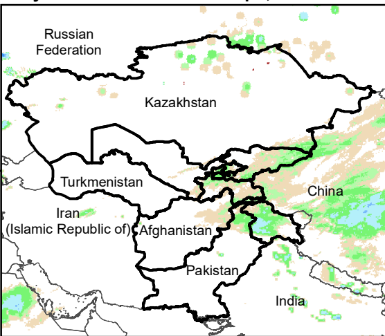
Daily Rainfall estimate for 11 Apr., 2004
