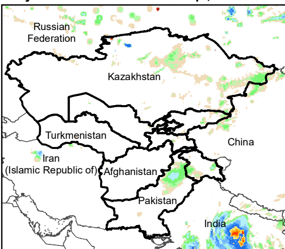
Daily Rainfall estimate for 20 Sep., 2004
