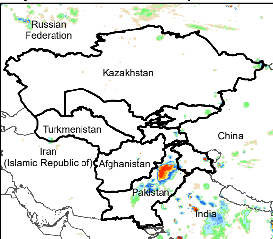
Daily Rainfall estimate for 19 Sep., 2004
