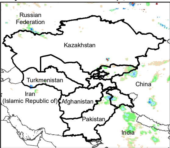
Daily Rainfall estimate for 18 Sep., 2004
