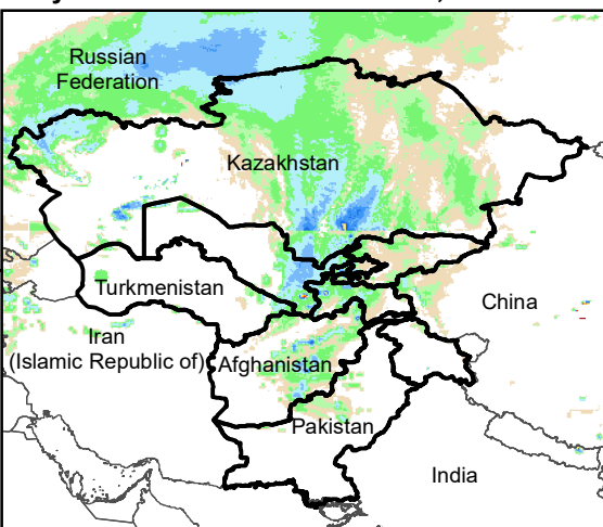
Daily Rainfall estimate for 25 Nov., 2004
