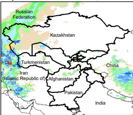
Daily Rainfall estimate for 26 Nov., 2004
