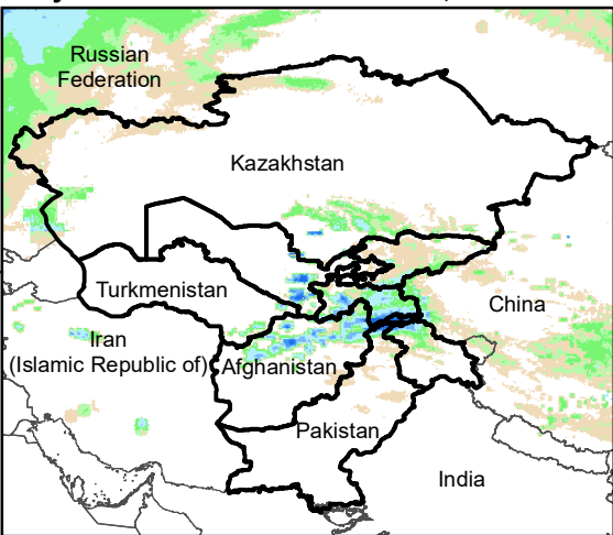
Daily Rainfall estimate for 24 Nov., 2004
